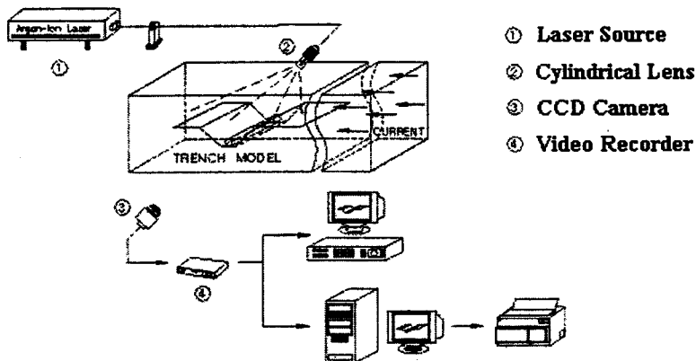
Fig. 4 Experimental setup for P.I.V. measurement
