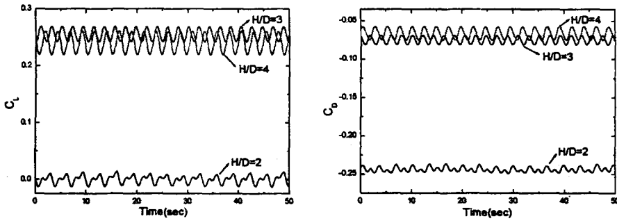
Fig. 10 Effects of cover depth ratio on C_D - C_L characteristics ( W/H=1.0 , \delta/H=0.1 , and Re_D=6 \times 10^3 )
