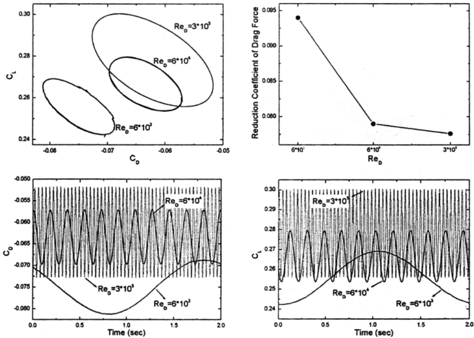
Fig. 7 Effects of Reynolds numbers on drag reduction coefficients, and C_D - C_L characteristics for \delta/H=0.1 , H/D=3 , W/H=1
